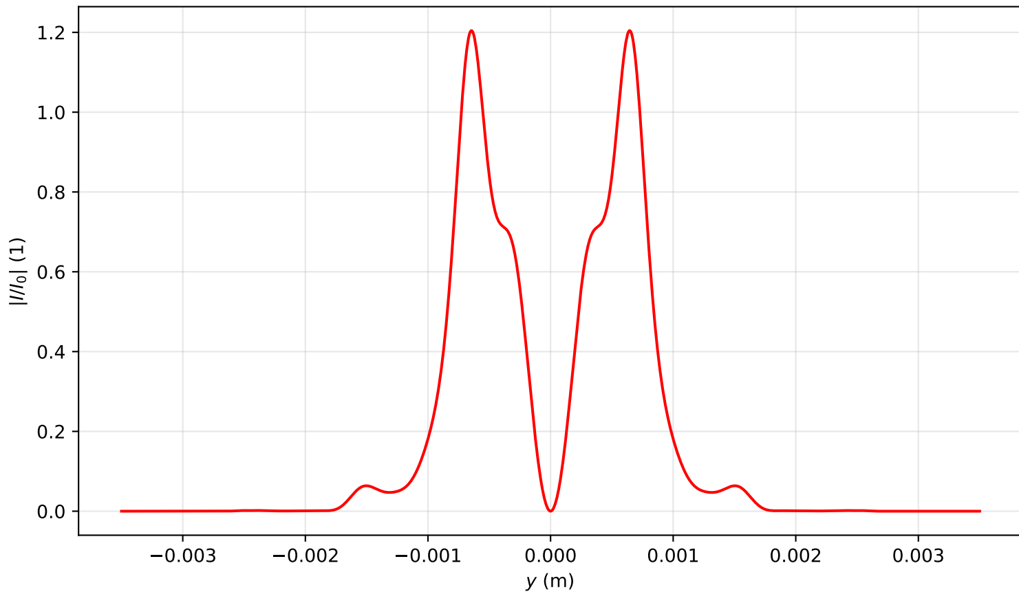
Intensity profile I(x=0, y, z=1.433)/I_0 , \text{Pin}=7.0\text{Pcr} , artificial time
